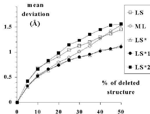
Figure 8 The mean deviation of atomic centres from their true positions after 800 cycles of free-atom refinement is shown as a function of the completeness of the starting model. The deleted atoms were chosen randomly from the whole structure (Fab plus water). The exact coordinates of the rest of the structure were used as the starting values. Different types of residual are compared: LS, standard least-squares (1); ML, the criterion marked as ML criterion in the CNS program; LS*, modified criterion (6); LS*1, criterion (42); LS*2, criterion (43).
