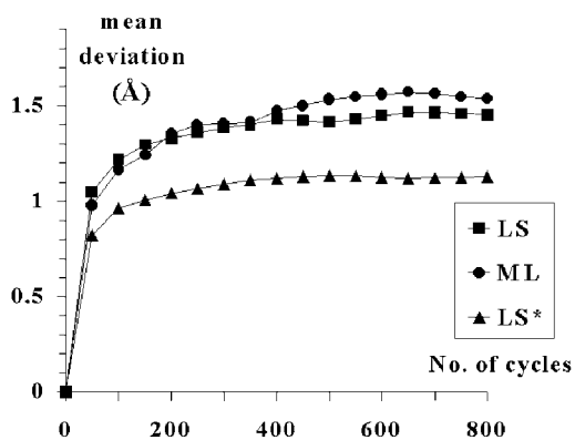
Figure 5 The mean deviation of atomic centres from their true positions in the course of the refinement starting from a 50% complete exact partial model: LS, standard least-squares (1); ML, the criterion marked as ML criterion in the CNS program; LS*, modified criterion (6).
