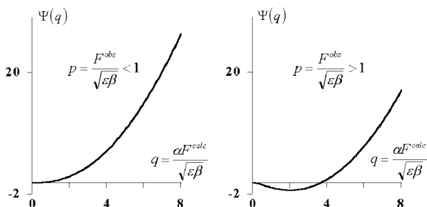
Figure 1 The behaviour of the target function \Psi in the residual (3)–(4) for relatively weak ( p = 0.7 , acentric, left) and relatively strong ( p = 2 , acentric, right) observed magnitudes. The modified observed magnitude p is defined as p = F_s^{\text{obs}}/\varepsilon\beta . The dependence on the modified calculated magnitude q = \alpha F_s^{\text{calc}}/\varepsilon\beta is shown.
