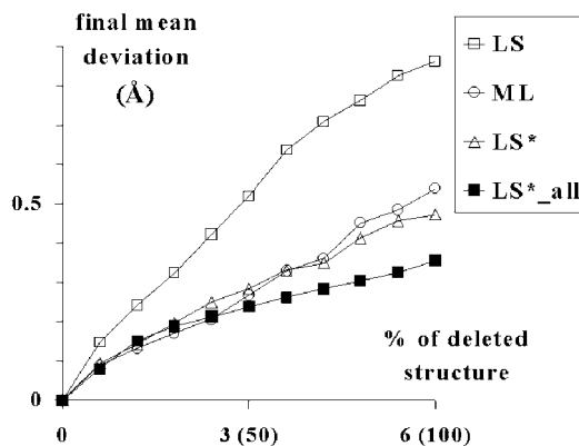
Figure 7 The mean deviation of atomic centres from their true positions after 800 cycles of free-atom refinement is shown as a function of the completeness of the starting model. The deleted atoms were chosen randomly from the water oxygen atoms only. The exact coordinates of the rest of the structure were used as the starting values. The figures in brackets indicate the percentage of deleted atoms with respect to all water oxygen atoms. Different types of residual are compared: LS, standard least-squares (1); ML, the criterion marked as ML criterion in the CNS program; LS*, modified criterion (6). A part of the LS* curve from Fig. 6 is shown (LS*_all) for comparison with the case when atoms are deleted from the whole structure and not from water molecules only.
