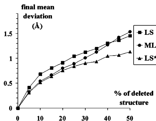
Figure 6 The mean deviation of atomic centres from their true positions after 800 cycles of free-atom refinement is shown as a function of the completeness of the starting model. The deleted atoms were chosen randomly from the whole structure (Fab plus water). The exact coordinates of the rest of the structure were used as the starting values. Different types of residual are compared: LS, standard least-squares (1); ML, the criterion marked as ML criterion in the CNS program; LS*, modified criterion (6).
